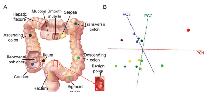
Figure 4. In vivo utilization of the novel REIMS endoscope system. A) Sampling points for three patients undergoing colonoscopy. B) Sampling points depicted on a three-dimensional PCA plot. The spectra acquired in vivo when the polyps were removed localize in a different part of space, whilst all other mucosal spectra are quasi-uniformly independent of the sampling location within the colorectal tract and the ileum.
