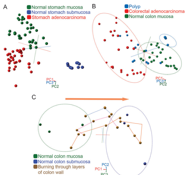
Figure 3. A) Three-dimensional PCA plot for healthy gastric mucosa ( n=32 ), gastric submucosa ( n=10 ), and adenocarcinoma of the stomach ( n=29 ) acquired from three patients ex vivo with a Xevo G2-S Q-ToF mass spectrometer. The differences between submucosa and the other two layers could potentially be used to develop a perforation risk-alert system for interventional endoscopy. B) Three-dimensional PCA plot for human colon adenocarcinoma ( n=25 , from seven patients) acquired from ex vivo samples, healthy colonic mucosa ( n=24 , from ten patients), and polyps ( n=13 collected from five patients) acquired from ex vivo endoscopy biopsies. The leave-one-patient-out cross-validation of the multivariate model containing spectra obtained by the analysis of normal and cancerous tissue resulted in 95% specificity and 88.5% sensitivity. The ellipsoids represent the polyps grouped with normal mucosa samples (green), cancerous samples (red), or separately (blue). C) Three-dimensional PCA plot containing 3 \times 3 normal, mucosal and submucosal sampling points and each scan acquired from three diathermy passes through the colonic layers ex vivo starting on the mucosal side (two patients). The arrow represents the direction of the diathermy pass and the consecutive scans are linked together with each burn. There is a clear shift observed from mucosa to submucosa.
