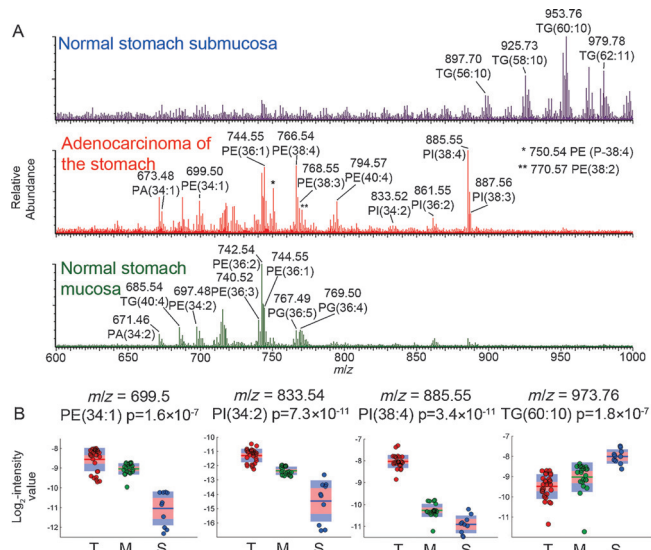
Figure 2. A) Mass spectra from gastric mucosa, gastric submucosa, and adenocarcinoma tissue recorded ex vivo using a modified Xevo G2-S Q-ToF mass spectrometer. Cancerous and healthy mucosal tissues feature mainly phospholipids in the m/z 600–900 region, whilst submucosa features triglyceride and phosphatidylinositol species in the m/z 850–1000 region. B) Comparison of the abundance of selected peaks showing significant differences between cancerous and healthy tissues in the range m/z 600–1000 using Kruskal–Wallis ANOVA, p < 0.005 . T = tumor, M = mucosa, S = submucosa.
